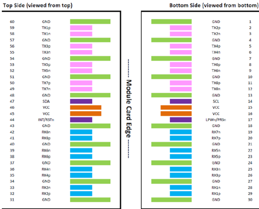
QSFP Pad Function Definition
