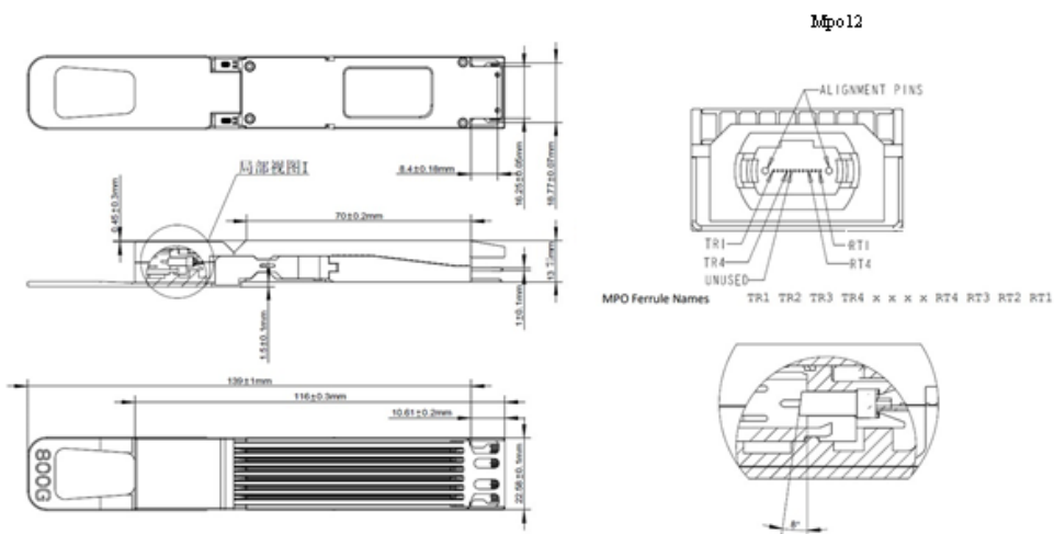
Mechanical Package Outline (All dimensions in mm)
